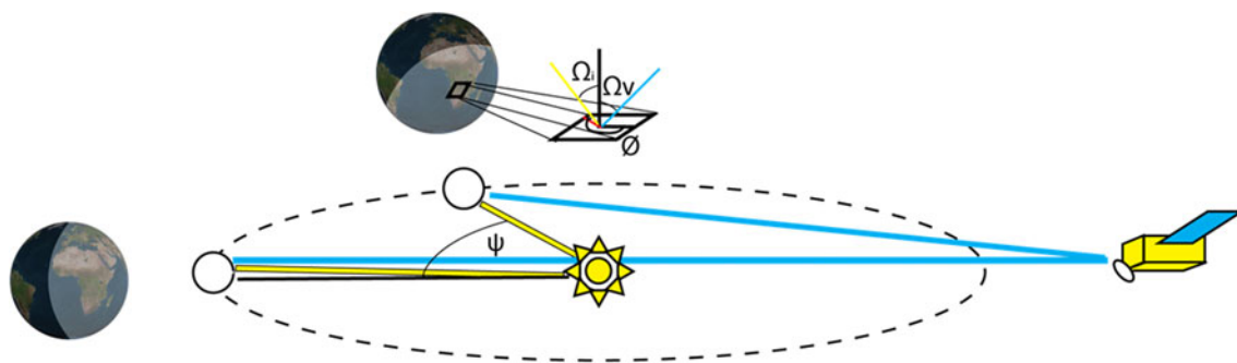
Fig. 1. Our conceptual design of a distant observer monitoring Earth and the change in backscattering as it revolves around the sun. \Theta is the azimuth angle, \Omega is the solar zenith angle, \Omega_v is the view angle and \Psi is the phase angle.
