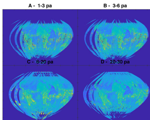
Fig. 6. All (including ocean and clouds) NDVI pixels from POLDER at the phase angles (a) 1–3°, (b) 3–6°, (c) 6–20° and (d) 20–30° aggregated and averaged from the 21-day period described in the Methods.
